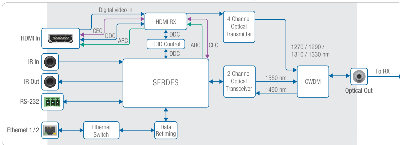
DVI-7366-TX Internal Block Diagram
