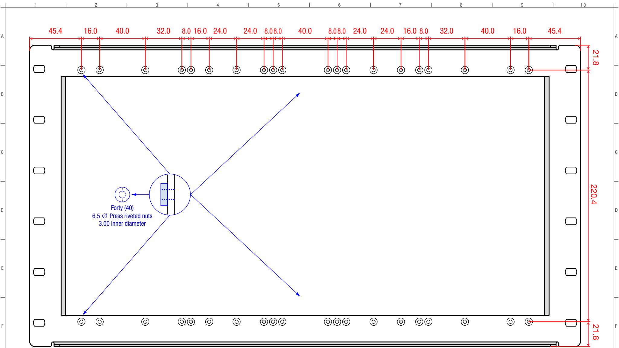
Bottom View
