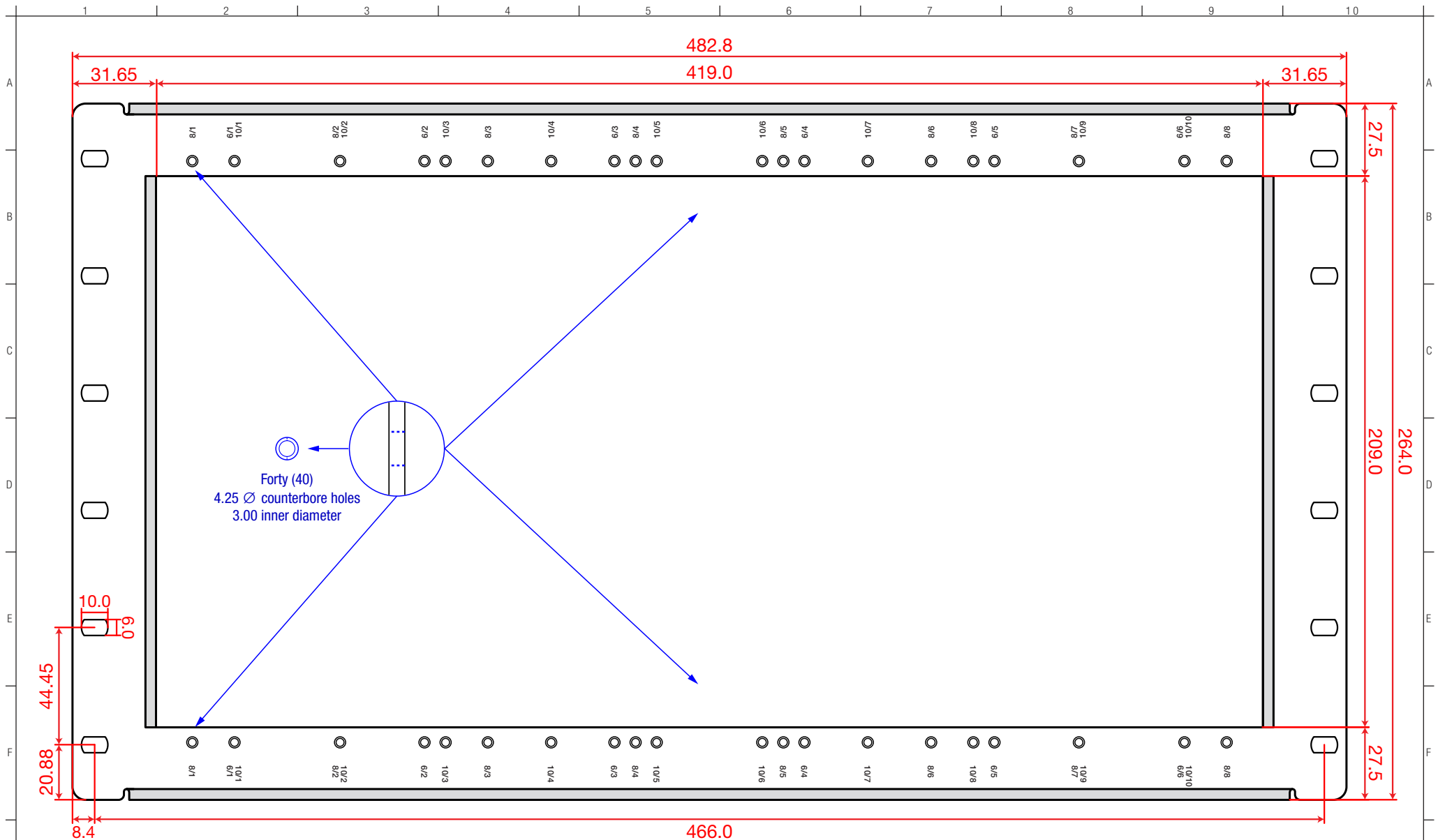
Front View
